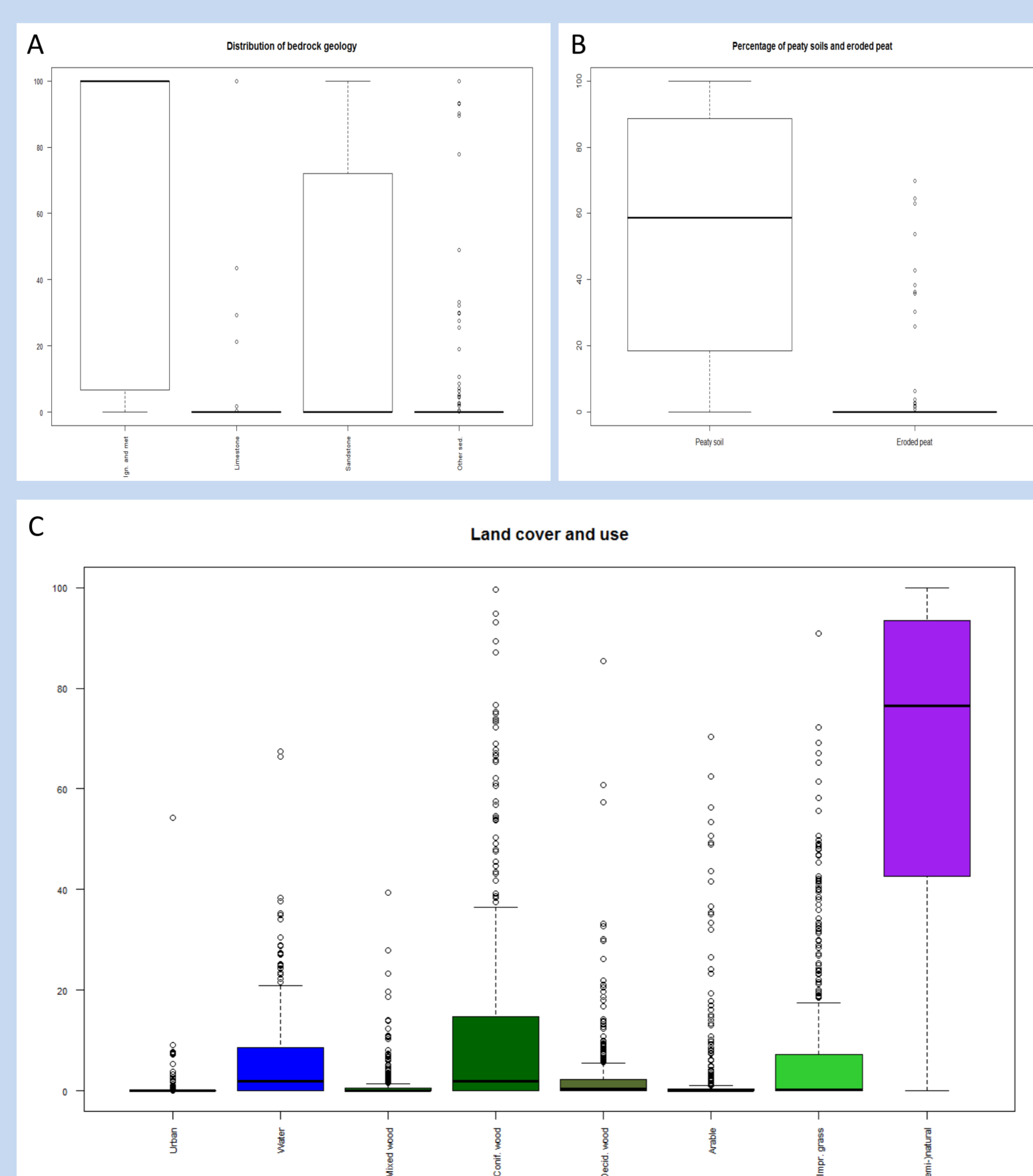
Figure 3: Distribution (percent cover in a catchment) of A. Type of bedrock geology, B. Distribution of peaty soil cover, and C. Land cover and use.
