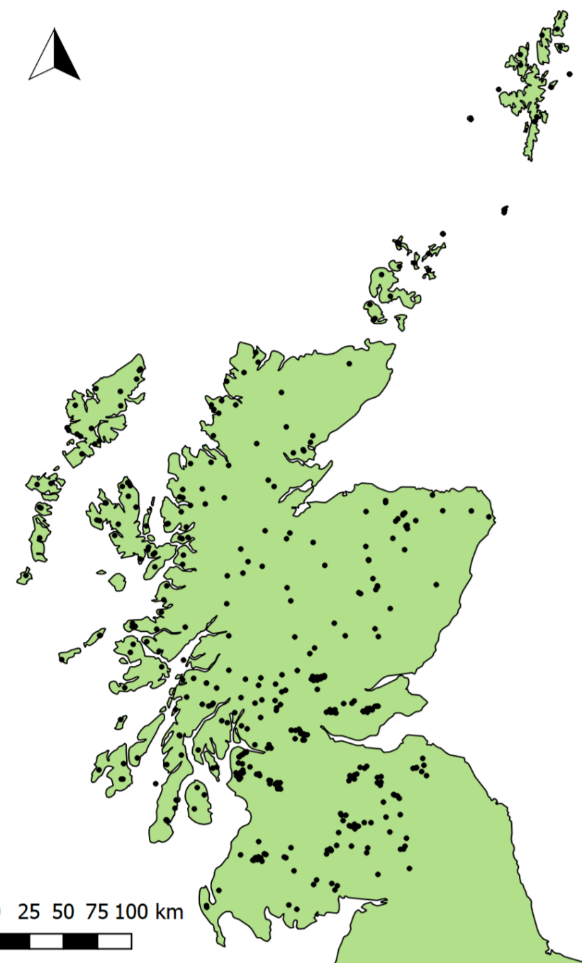
Figure 1: Location of drinking water catchments in Scotland.
