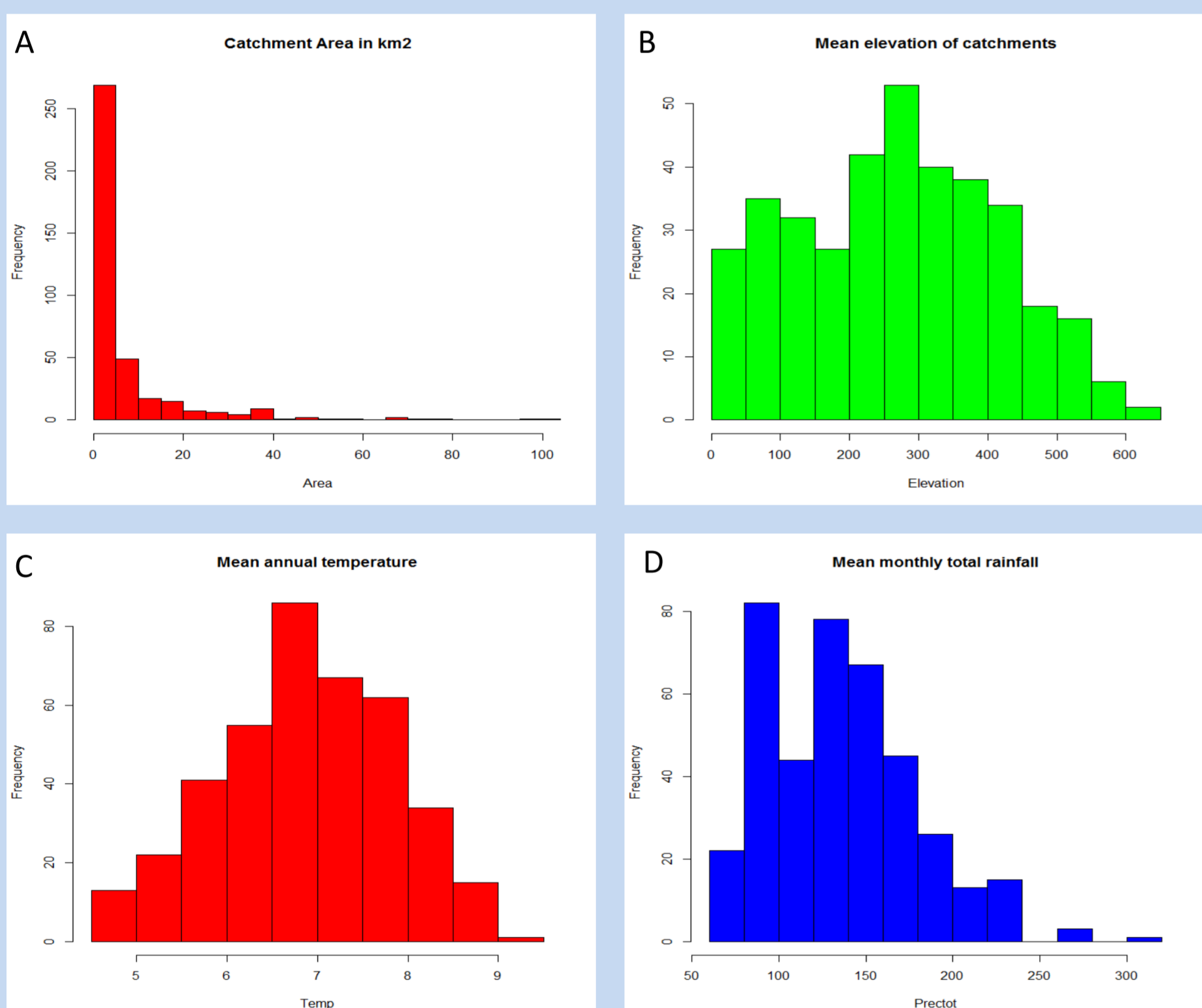
Figure 2: Histograms of A. Catchment size in km 2 . Catchments above 100 km 2 in size have been omitted (16), B. Mean elevation of catchments, C. Mean annual temperature in °C per catchment, and D. Mean monthly rainfall in mm per catchment.
