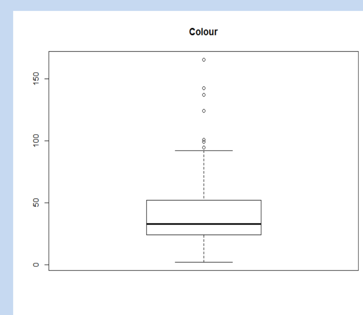
Figure 4: Distribution of median catchment values for colour (in mg/l Pt/Co).
