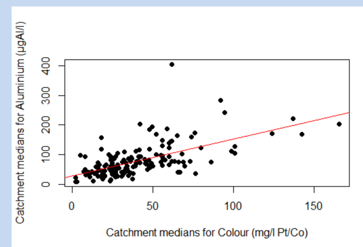
Figure 5: Catchment median aluminium concentration plotted against catchment median colour concentration, with a fitted regression line.
