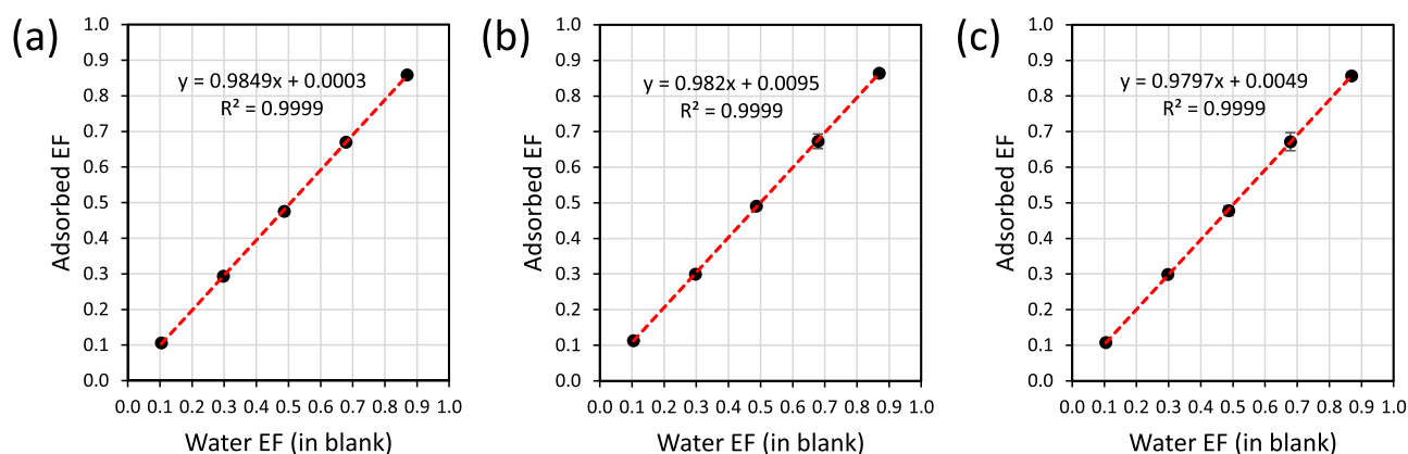
Fig. 3. Influence of fluoxetine enantiomeric fraction in 0.01 M \text{CaCl}_2 buffer at pH 7.5 (x-axis) on the enantiomeric fraction of fluoxetine adsorbed to bioplastic (a), polyamide (b) and cellulose (c) particulates (y-axis).
